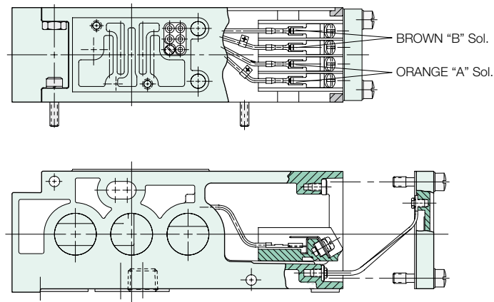
Mark 8 FlexiBlok with Terminal Block: OPTION 19tM
